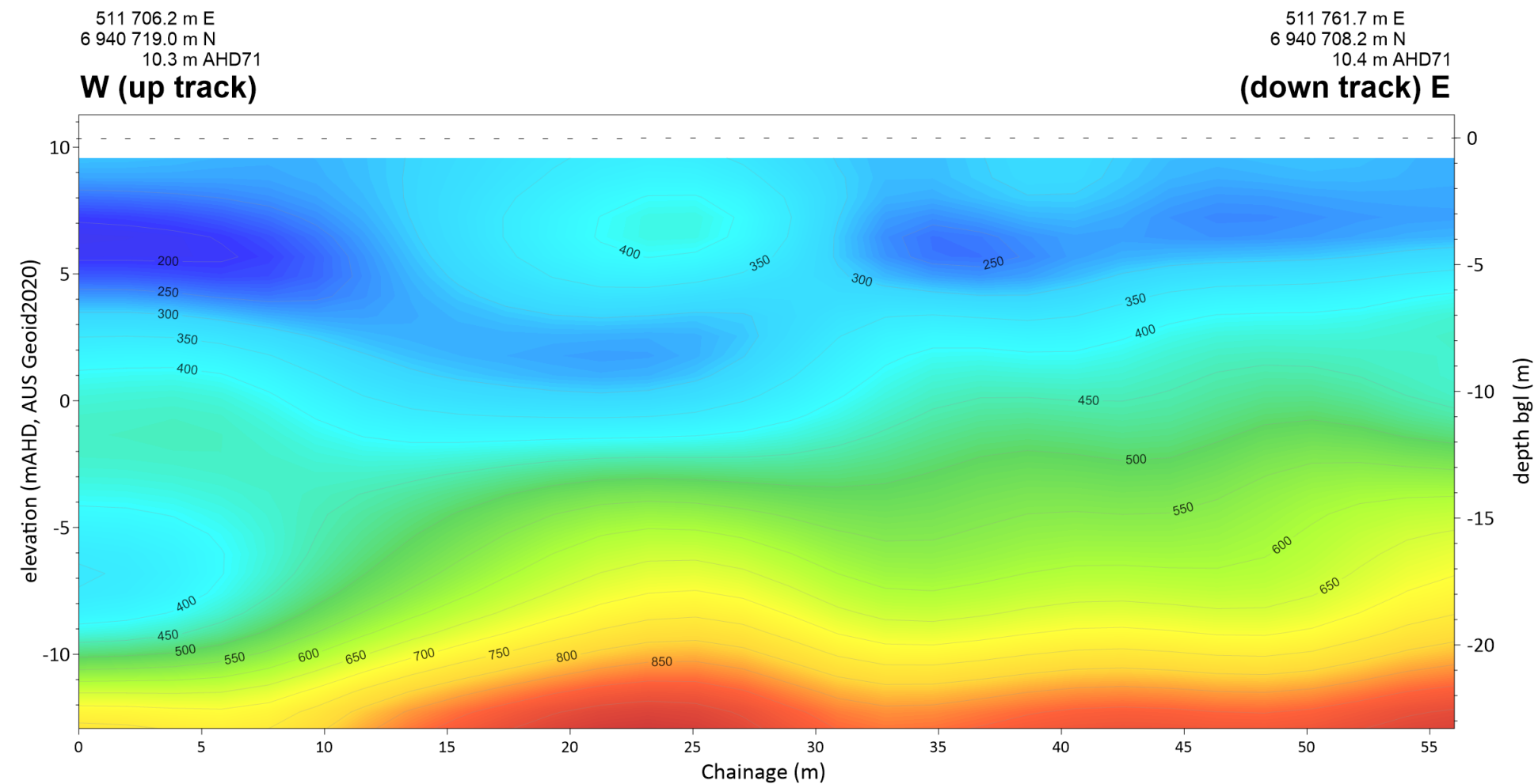
Seismic Line MASW AU-GP 141
